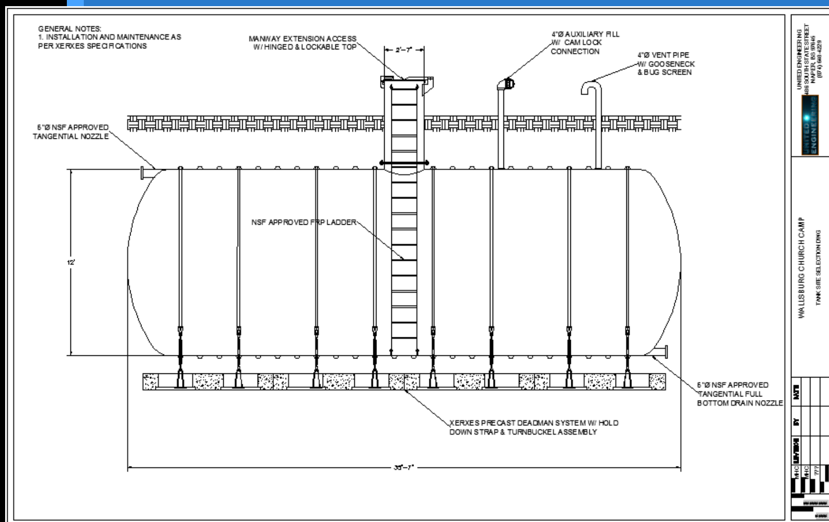
Xerxes Fiberglass Tank
