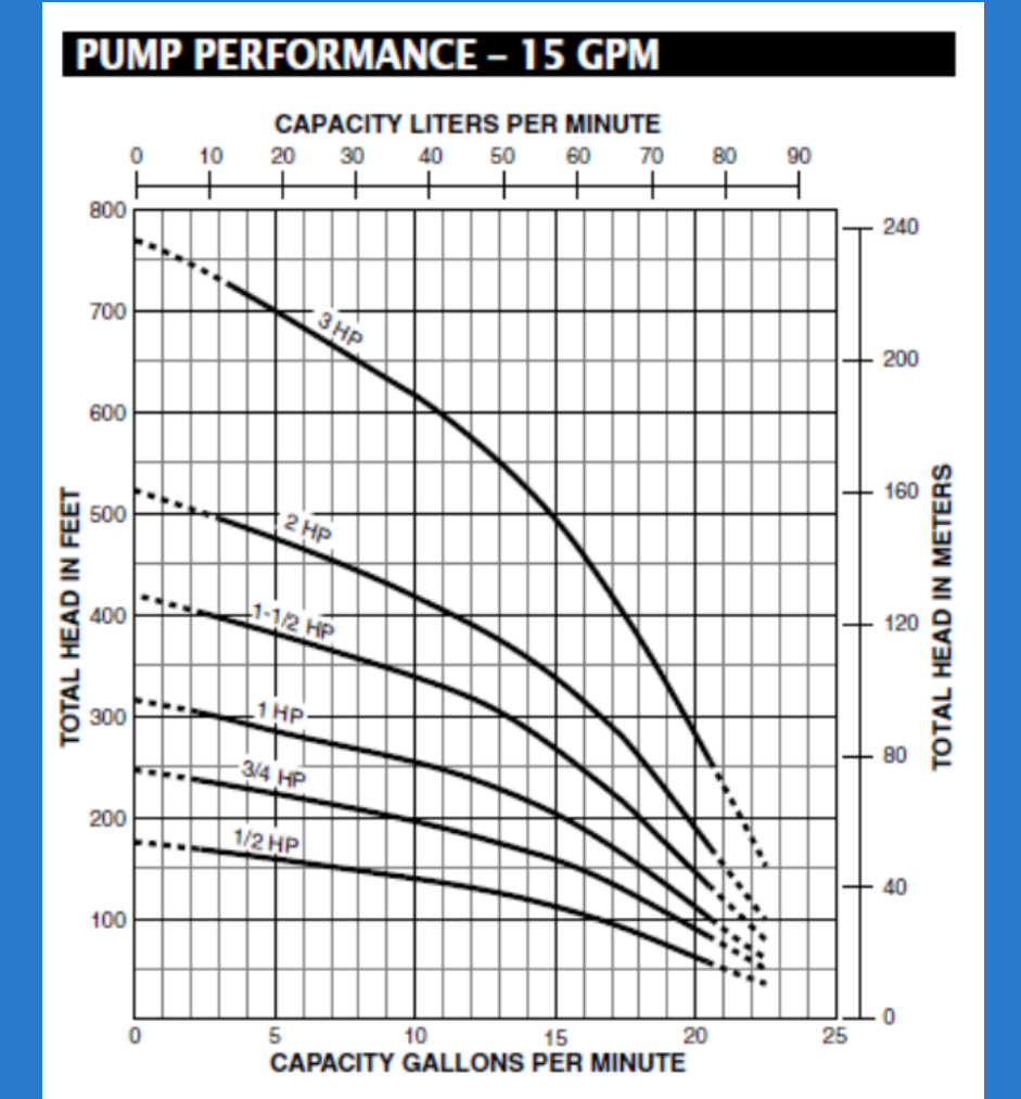
STA-RITE 4" Submersible HS Series Pump
