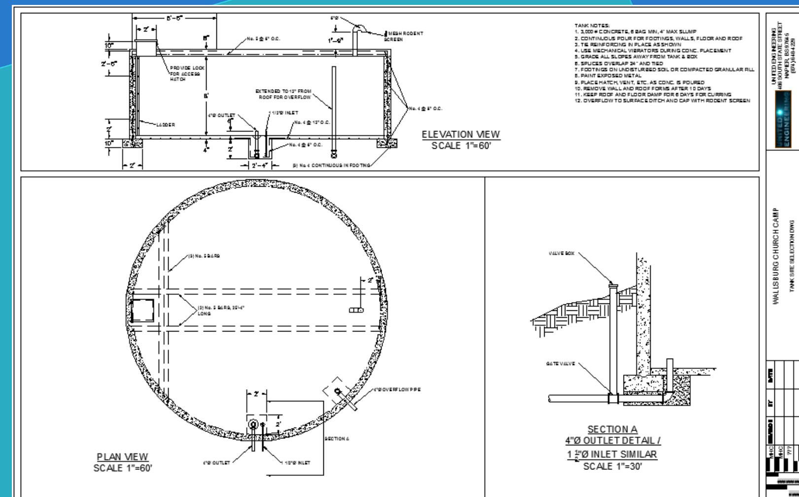
Reinforced Concrete Tank
